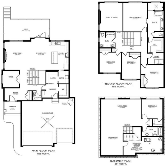
2 STOREY - 2540 SQ.FT.
